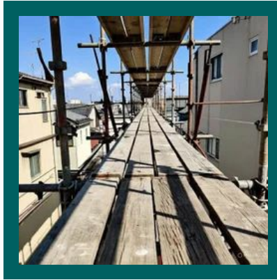
Scaffold Walkway Plank
